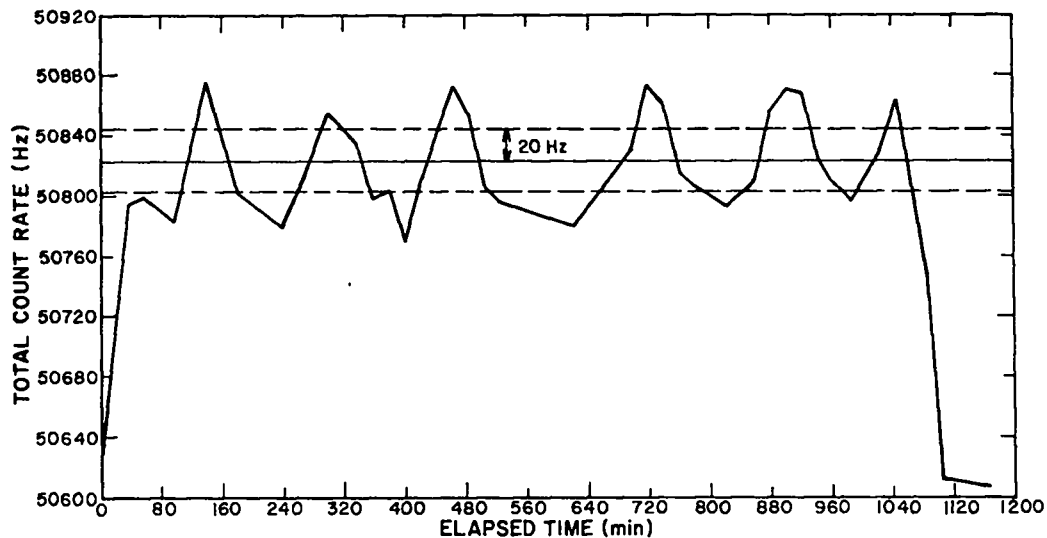
Fig. 12. Count rate record for stability experiment conducted on December 1-2 using all detectors for 1100 min. Results fall within a 20-Hz error band.
